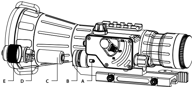
FIGURE 3-1. CO-LR BATTERY INSTALLATION
