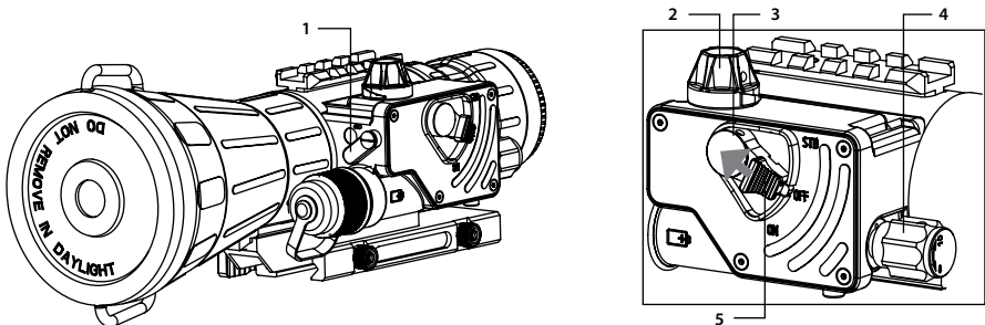
FIGURE 3-12. CO-LR CONTROLS
