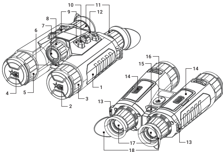
FIGURE 1-1. MAIN PARTS
