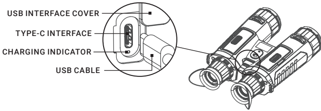
FIGURE 2-5. CABLE CONNECTION
